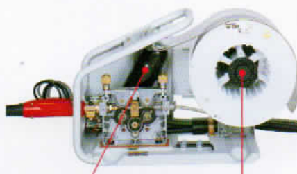
Encoder motor Wire spool shaft with brake
